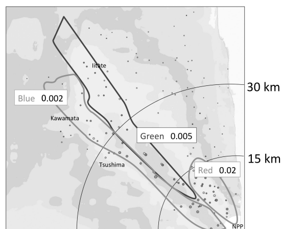
Fig. 1 Distribution map of ^{110m}\text{Ag}/^{137}\text{Cs} ratio divided by three groups based on the ratio.
