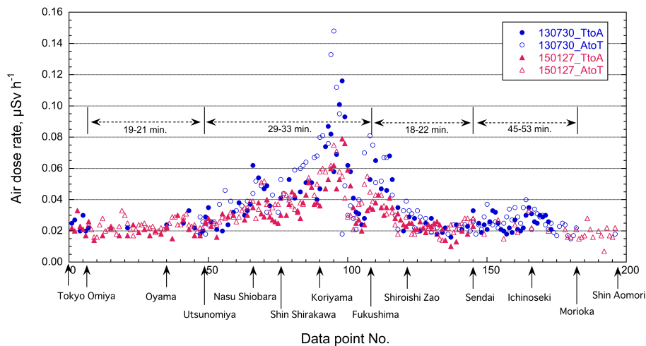
Fig. 1. Air dose rate in Shinkansen super express train between Tokyo (T) and Shin-Aomori (A) Stations measured on 30 July 2013 and 27 January 2015 with a handheld radiation monitor.
